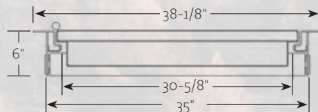
Standard Door Dimensions - Top View
