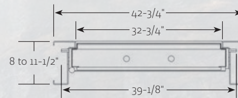
Clamshell Door Dimensions - Top View
