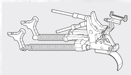
Reverse Striker Mechanical Trigger
