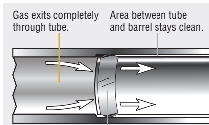
Gas exits completely through tube. Area between tube and barrel stays clean. Invector-DS tubes have a special brass seal with multiple cuts that compresses against the barrel wall and completely seals against gas leakage.
