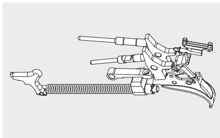
Reverse Striker Mechanical Trigger
