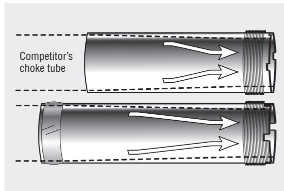
Longer overall length, as much as 1-1/8" over a leading competitor, allows a more gradual choke taper on Invector-DS tubes for denser shot patterns, better pattern percentages and faster shot velocities.
