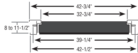
Clamshell Door Dimensions - Top View
