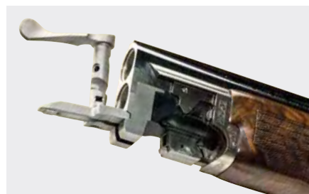
Locking Bolt and Hinge Pin
