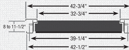
CLAMSHELL DOOR DIMENSIONS - TOP VIEW
