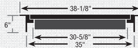
STANDARD DOOR DIMENSIONS - TOP VIEW
