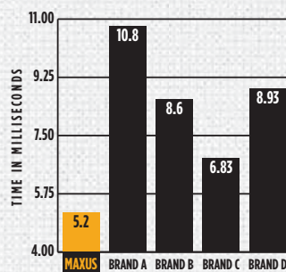
Locktime Comparison
