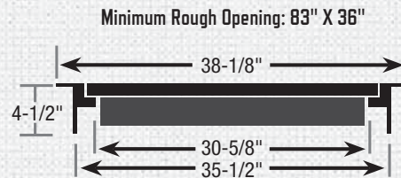
SECURITY DOOR DIMENSIONS - TOP VIEW
