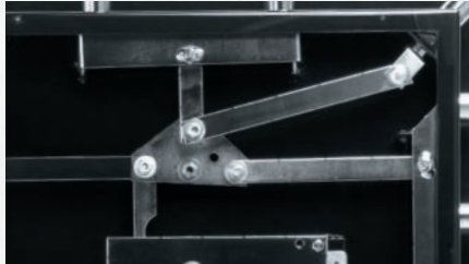
UNI-FORCE LOCKING SYSTEM Robust cam locks and a multiple diversion bar system divert pressure from reaching the lock.
