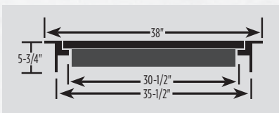
OUT-SWING DOOR DIMENSIONS - TOP VIEW
