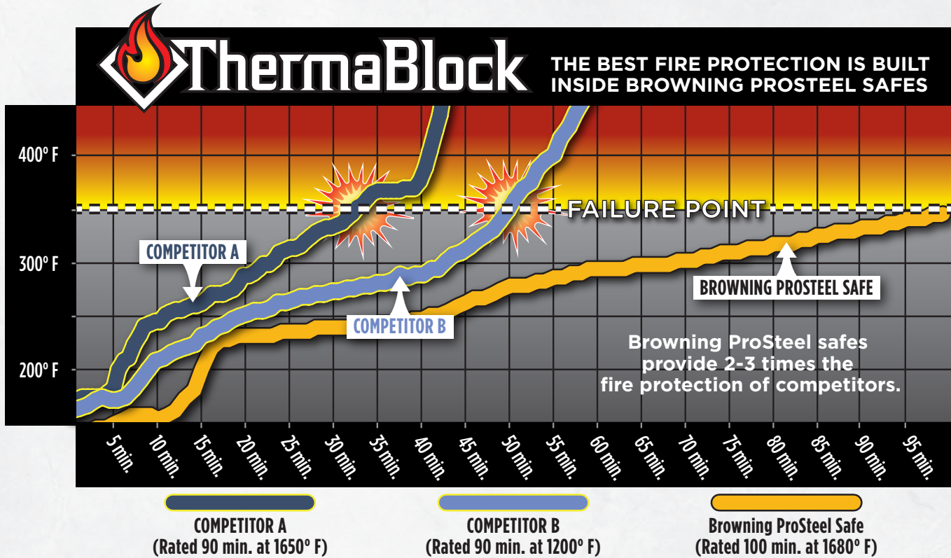
This graph compares a Browning ProSteel safe with ThermaBlock and external hinges to a pair of comparable safes from leading competitors with internal hinges.
