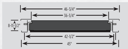
IN-SWING DOOR DIMENSIONS - TOP VIEW
