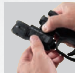
The rail bracket remains on the MIL-STD 1913 Picatinny rail of the firearm. The EDC Light Module instantly mounts to the rail.
