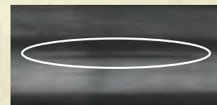
The competitors' choke tube is grooved and pitted after shooting 500 rounds of steel shot.
