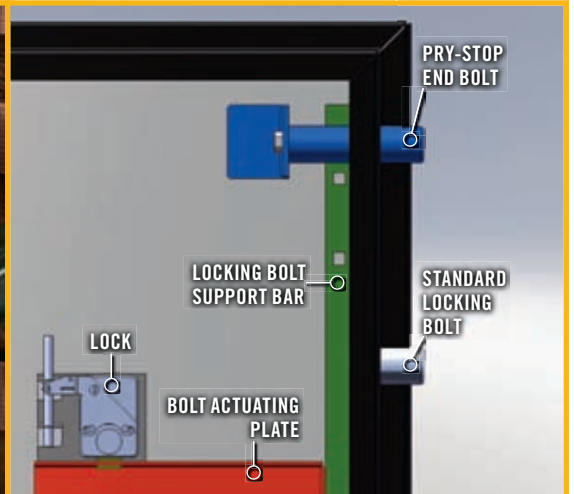
Pry-Stop End Bolt Mechanism
