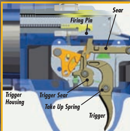
Full sear engagement (Ready to fire)
