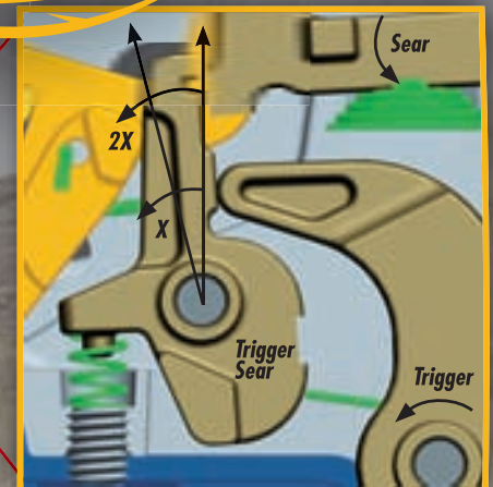
Close-up of unseared (Fired)
