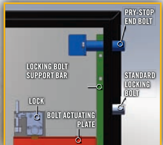
Pry-Stop End Bolt Mechanism
