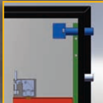
Pry-Stop End Bolt Mechanism
